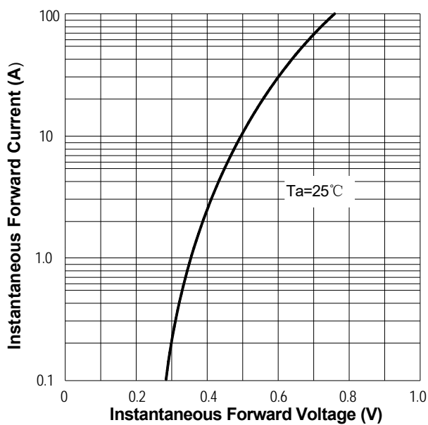
FIG.3: Forward Voltage
