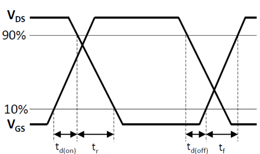
Figure 21. Switching Times Definition
